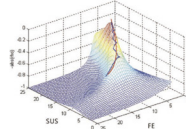
Software algorithm
